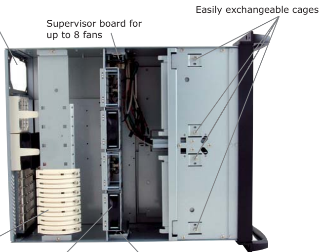
Cage with anti-vibration and filter for 3x3½" HDD
