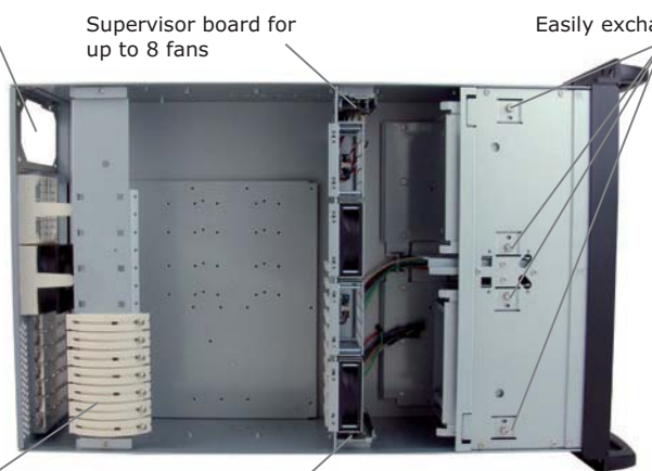
Easily exchangeable fan holder rail and fan holders
